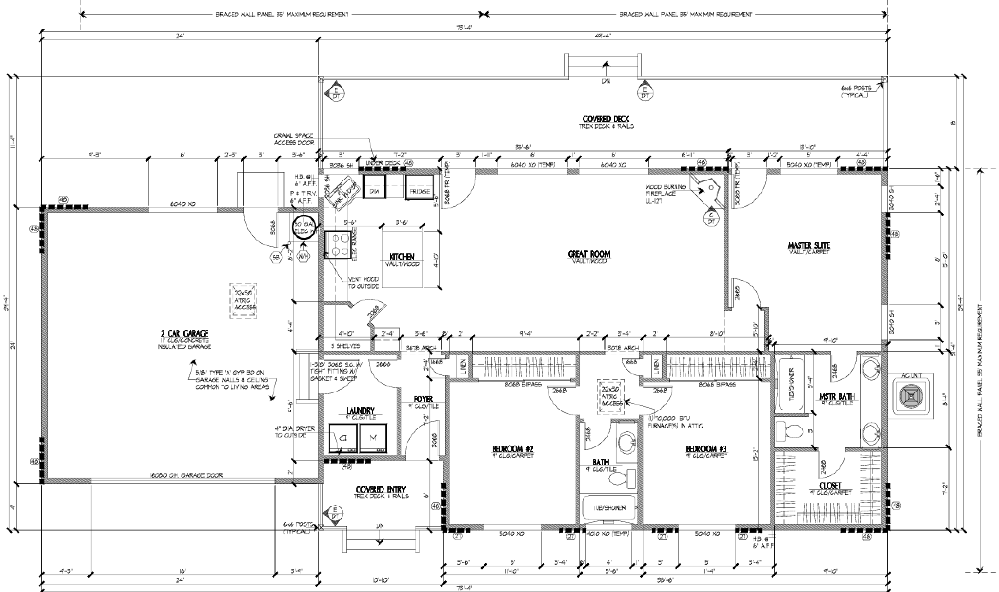
FLOOR PLAN
